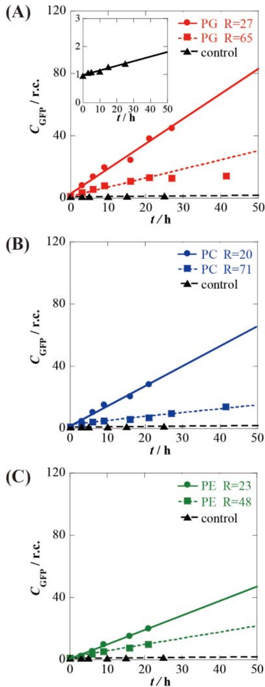
Figure 2 | Time-courses of the GFP concentration per unit volume, C_{\text{GFP}} , in small (radius R \sim 20 \mu\text{m} ; circle) and large ( R > \sim 50 \mu\text{m} ; square) droplets coated by a lipid layer of (A) DOPG, (B) DOPC, or (C) DOPE, respectively. C_{\text{GFP}} of the bulk solution is shown as a control (triangle). These data fit linear lines from 0 to 20 h, and C_{\text{GFP}} at 3 h in the bulk solution is taken as unity for all of the graphs.
