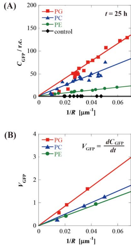
Figure 3 | The size-dependence of (A) the GFP concentration per unit volume C_{\text{GFP}} at 25 h, and (B) the production rate V_{\text{GFP}} from 0 to 20 h, evaluated from the slope of linear increase on C_{\text{GFP}} . The lipids are DOPG (square), DOPC (triangle), DOPE (circle), and the bulk solution as a control (diamond).
